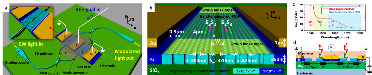
Fig. 1. (a) A 3D perspective of an EO polymer filled silicon slot PCW MZI modulator designed on an SOI substrate. (b) A tilted view of the lattice-shifted PCWs on one arm of the MZI. (c) Simulation result of engineered group index (red curve) in the slot PCW as a function of wavelength, showing 8nm low-dispersion slow-light optical spectrum. Also overlaid is the dispersive group index (blue curve) for non-band-engineered PCW for comparison. HD SL: high-dispersion slow-light; LD SL: low-dispersion slow-light; LD FL: low-dispersion fast-light. (d) Equivalent circuit of the MZI modulator in a push-pull configuration, with a constant gate voltage applied on the backside silicon substrate.
