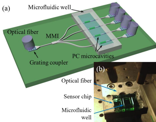
Fig. 2. (a) Schematic of the PC microcavity biosensor array. (b) The sensor chip on a fiber coupling test stage.
