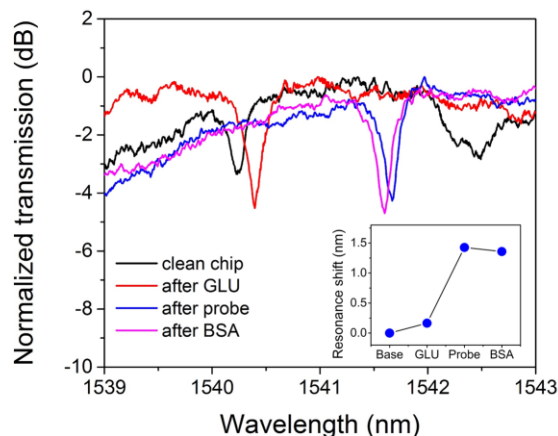
Fig. 4. Transmission spectra of a L13 with nanoholes before and after functionalization. Inset shows the resonance shift at each step. GLU: glutaraldehyde; probe: anti-gentamicin antibody; BSA: bovine serum albumin.
