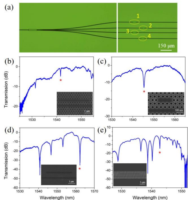
Fig. 3. (a) Stitched microscope image showing the MMI coupler and four PC sensors on the four channels. (b)-(e) Transmission spectra and SEM images of PC microcavities side-coupled to PC waveguides: (b) L13 with nanoholes, (c) L3, (d) L55. Red star markers show the resonance dip used for biosensing test.
