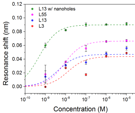
Fig. 5. Resonance shift of the four devices combined in the sensor array when target gentamicin antibiotics were bound to anti-gentamicin antibody on the sensor surface. The colored background and lines indicate the detection range for different PC microcavity biosensors.
