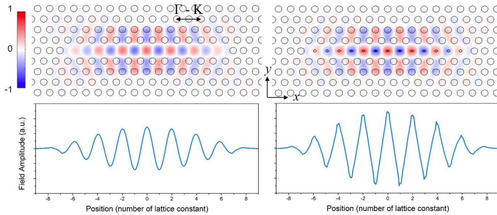
Fig. 1. Mode profiles ( E_y ) of L13 and L13 with nanoholes PC microcavities.
