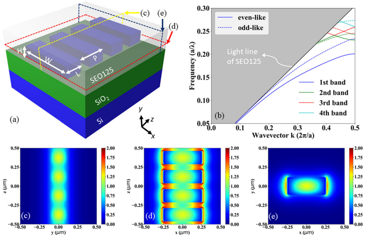
Figure 1. a) Schematic of an SWG waveguide for the optical modulator. b) Photonic band structure of SWG waveguides with SEO125 as top cladding for the waveguide width W = 500 \text{ nm} and pillar length L = 175 \text{ nm} . The black line at the boundary of the grey region indicates the light line of SEO125. The solid and dashed lines indicate the even-like and odd-like modes respect to the central slab plane in the y -direction, respectively. The electrical field distribution of the SWG waveguide at c) x -slice ( x = 0 \text{ }\mu\text{m} ), d) y -slice ( y = 0 \text{ }\mu\text{m} ), and e) z -slice ( z = 0 \text{ }\mu\text{m} ), for the SWG waveguide width W = 500 \text{ nm} , pillar length L = 175 \text{ nm} , height H = 220 \text{ nm} , and period P = 250 \text{ nm} .
