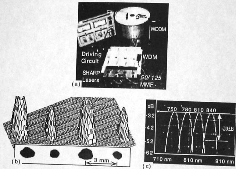
Fig.2 (a) The four channel WDM/WDDM light transmitting and receiving module picture, (b) The four output spots of the four channel WDDM, (c) The optical spectrum of the four wavelengths used in the WDM/WDDM system.
