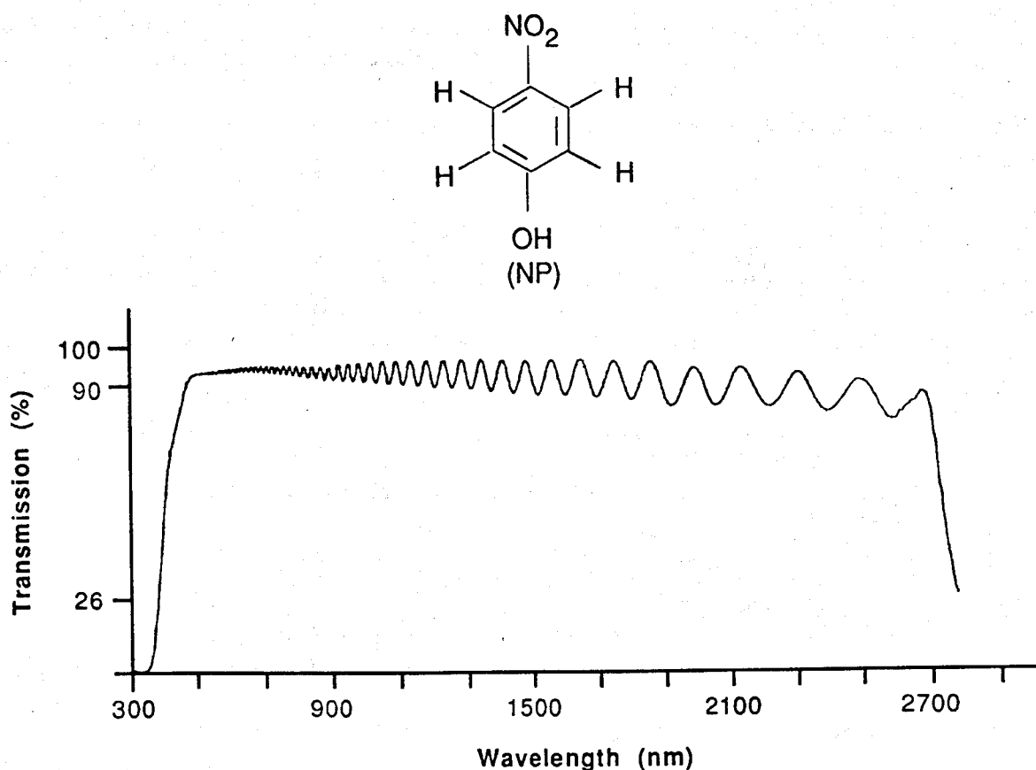
Figure 2 The Transmission Spectrum of 10 \mu\text{m} Nitrophenol/Gelatin Thin Film.
